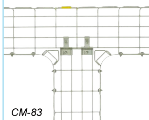
Ngã Ba (R=75mm)
